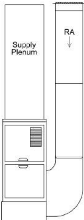
Model No. 148NF 20x25 to 12x25 Elbow Boot
