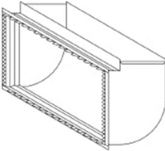
Model No. 248 1" Top Filter Access
